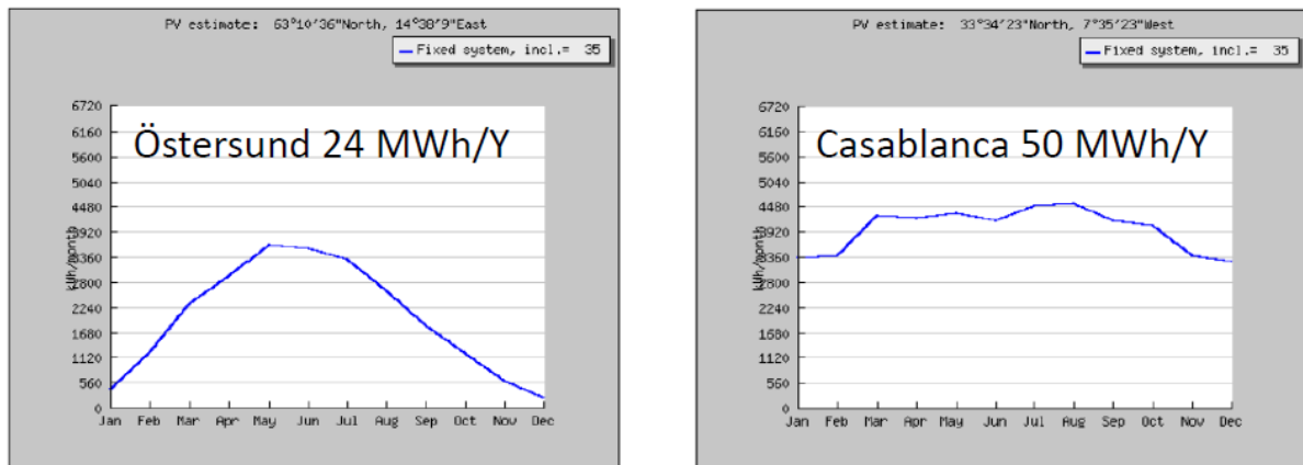
Figure 5 Simulated power generation as monthly energy output from a 28 kW photovoltaics installation in Östersund and Cassablanca (28 kW installation corresponds to photovoltaics installed at the roof of the Mid Sweden University and was therefore used in the simulation to compare real output with data from the simulation).
