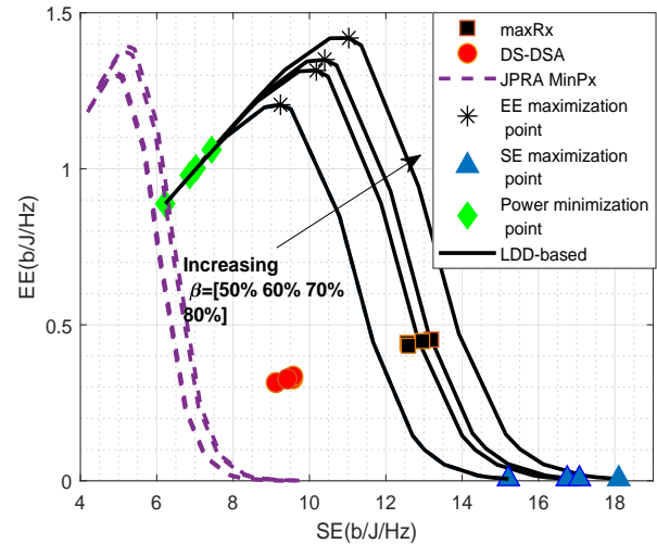
Fig. 4: Energy-efficiency versus spectral-efficiency with \chi = 50\% and \beta = [50\% \ 60\% \ 70\% \ 80\%] at the measuring time interval t_5 , average traffic load L_{DBS} = [50\% \ 30\% \ 30\% \ 60\% \ 20\% \ 30\%]
