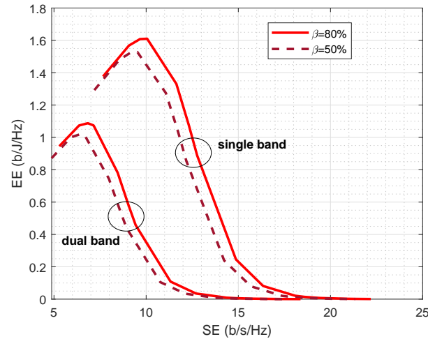
(a) SE versus EE comparison for single-band and dual-band scenarios; \chi = 50\%
