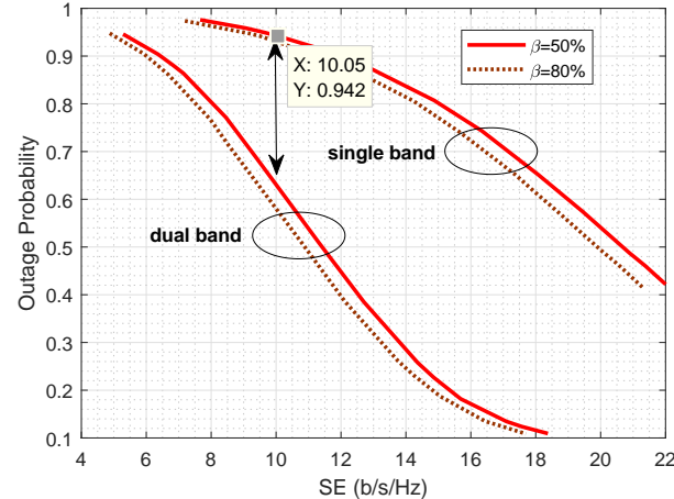
(b) Outage probability comparison between single-band and dual-band scenarios; \chi = 50\%
