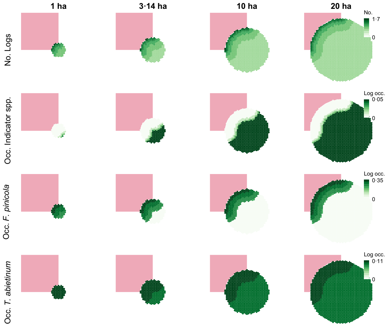
Fig. 2. Starting conditions predicted by models at t < 10 years under current forestry management conditions; that is 25% of the forest fragment edge adjacent to a clear-cut (pink square). The colour scale of each cell ( 140 \text{ m}^2 sample units) shows the median value of the posterior distribution of the number of logs (no. logs) or occupancy of logs (Occ.) by indicator species, Fomitopsis pinicola and Trichaptum abietinum .
